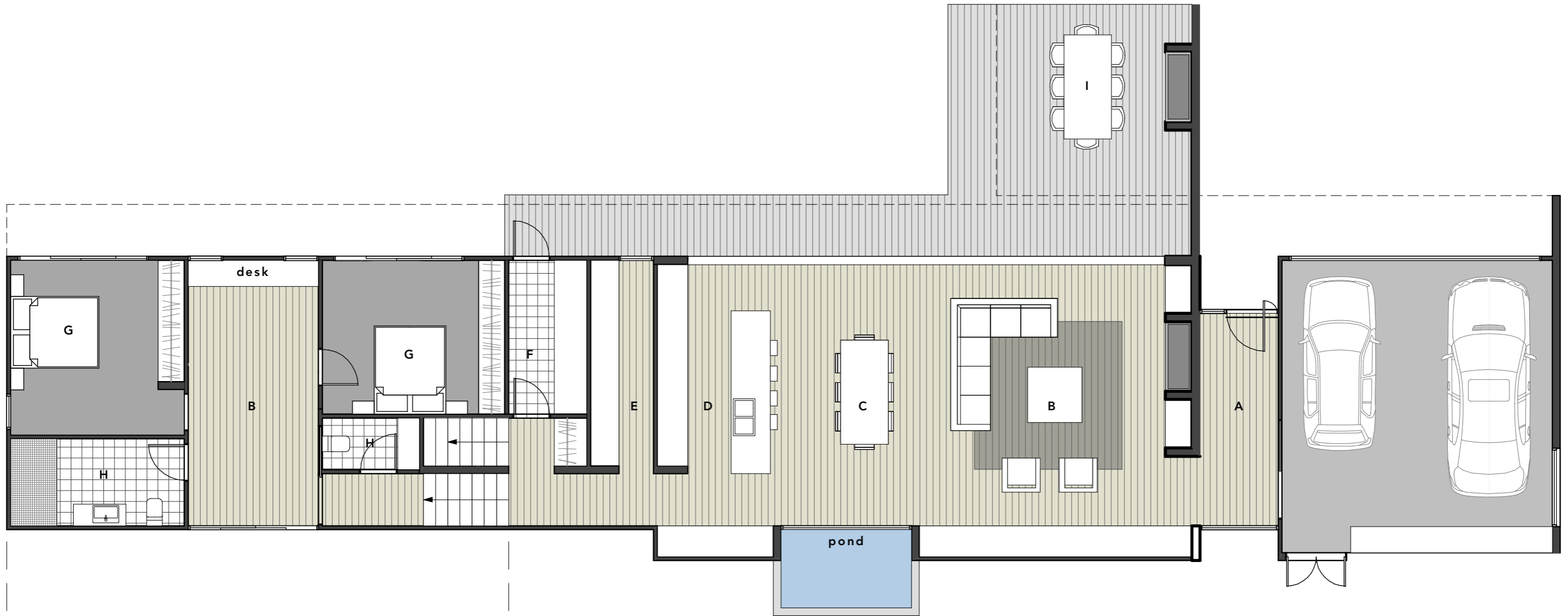
WHANAU floor plan
